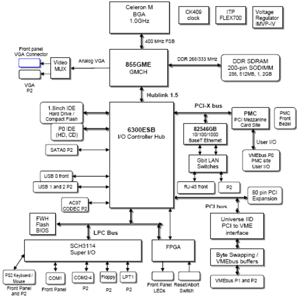
Figure 1-1 XVME 689-VR7 Block Diagram
