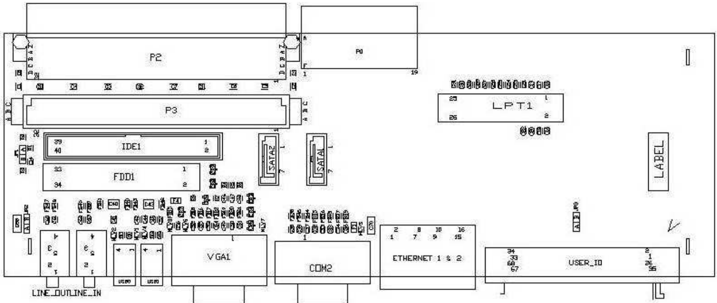
Figure 5-1 XVME-990/X Installation (XVME-990-001 shown)
