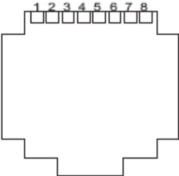
Figure 2-11 RJ-45 Serial Port Connectors
